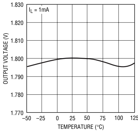
Output Voltage
