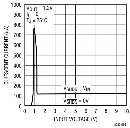
Quiescent Current
