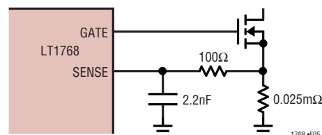
Figure 5. Sense Pin Filter
