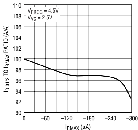
I_{DI01/2} to I_{RMAX} Ratio vs R_{MAX} Current
