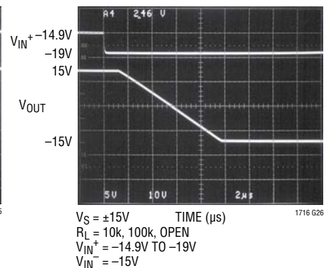
Below V_S^- Fault (Falling)
