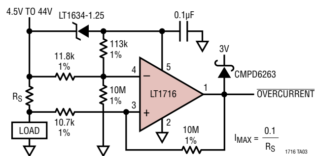
Overcurrent Flag
