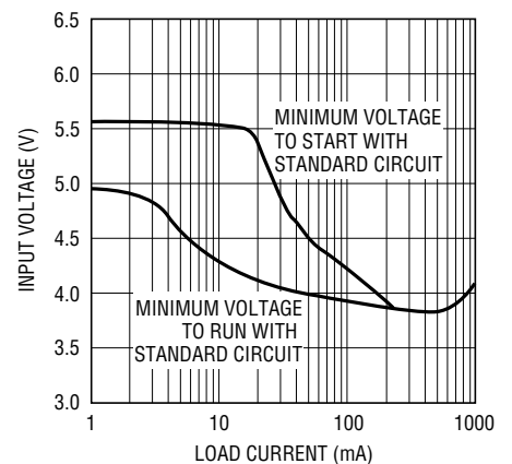
Minimum Input Voltage with 3.3V Output
