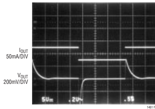
Figure 2. 50mA Load Step with C L = 2μF
