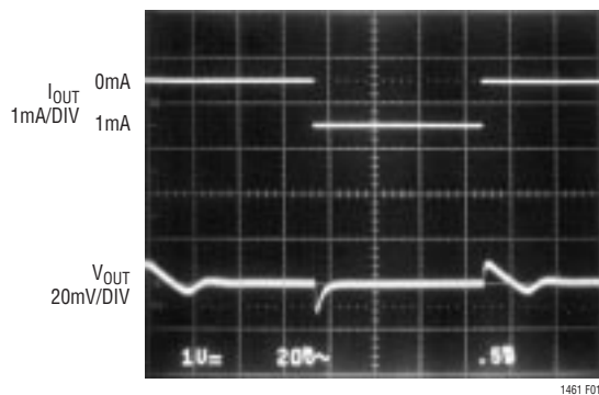
Figure 1. 1mA Load Step with C L = 1μF
