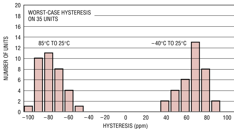
-40°C to 85°C Hysteresis
