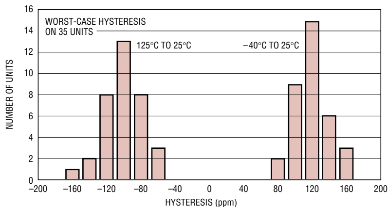
-40°C to 125°C Hysteresis
