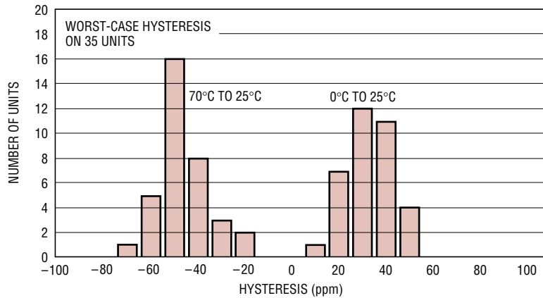
0°C to 70°C Hysteresis
