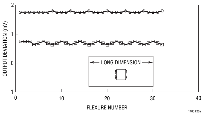
Figure 20a. Two Typical LT1460S8-2.5s, Vertical Orientation Without Slots
