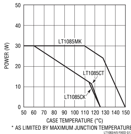
LT1085 Maximum Power Dissipation*
