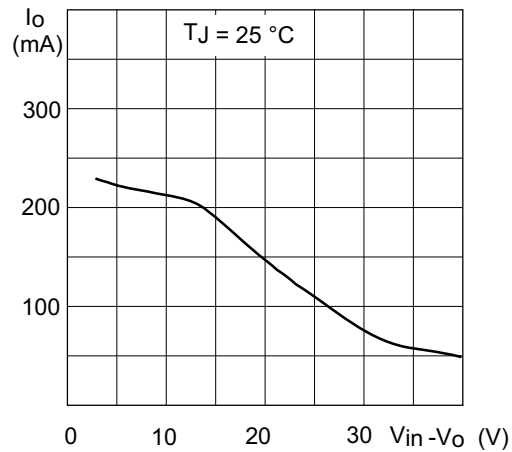
Figure 4. Current limit
