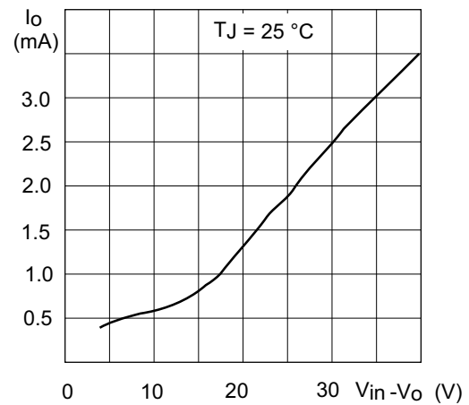
Figure 5. Minimum operating current
