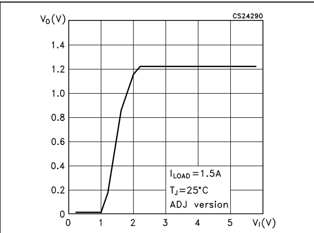
Figure 14. Output voltage vs input voltage
