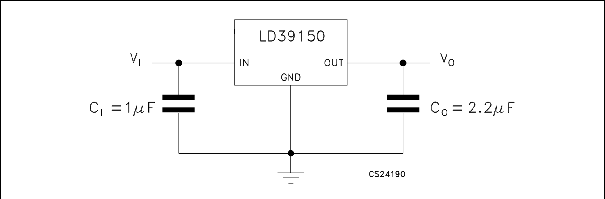
Figure 5. LD39150 DPAK
