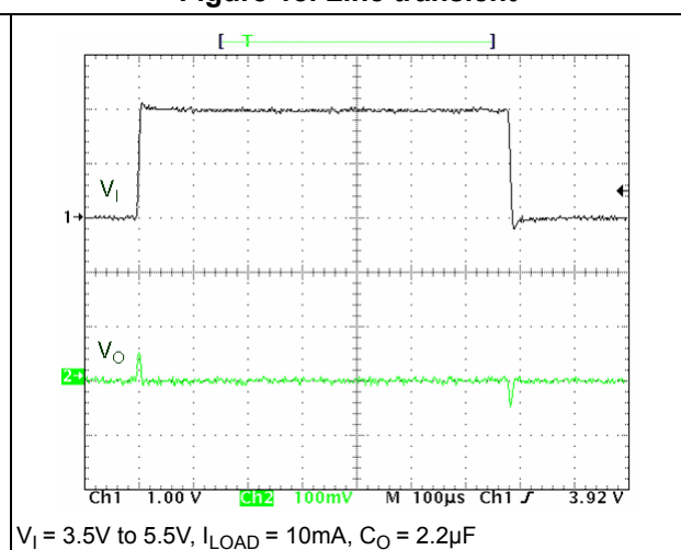
Figure 18. Line transient
