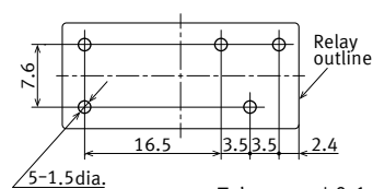
Recommended PC board pattern (BOTTOM VIEW)
