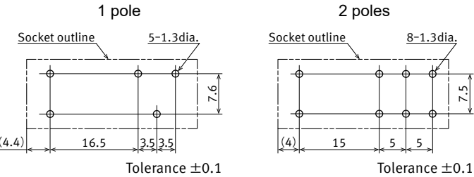
Recommended PC board pattern (Copper side view)
