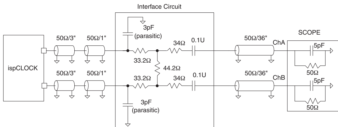
Figure 5. LVDS/LVPECL Termination Load
