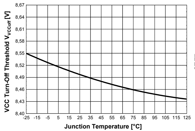
Figure 27 VCC Turn-Off Threshold V_{VCCoff} vs. T_j
