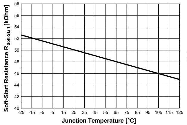
Figure 39 Soft-Start Resistance R_{Soft-Start} vs. T_j
