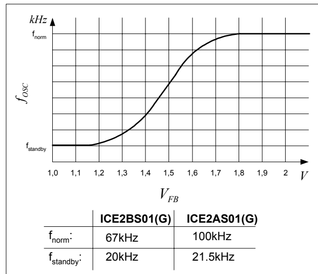
Figure 12 Frequency Dependence
