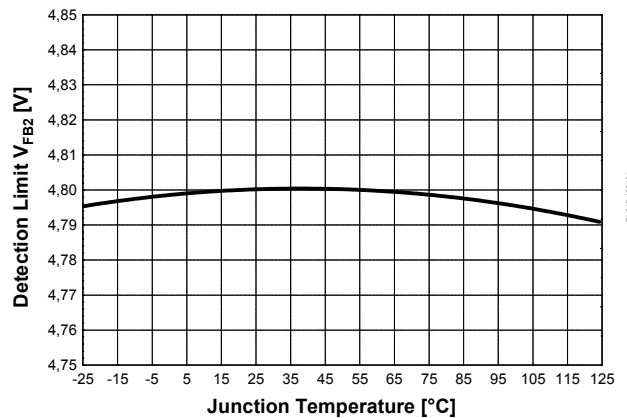
Figure 40 Detection Limit V_{FB2} vs. T_j
