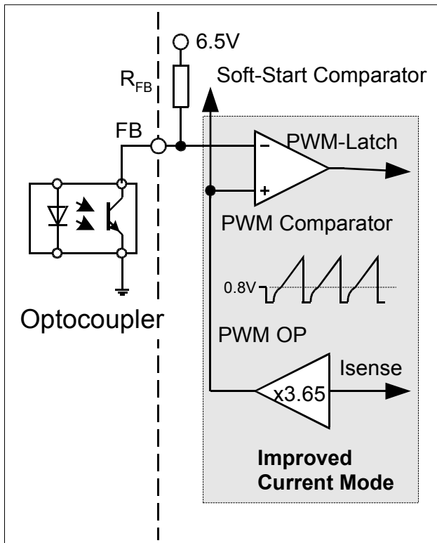
Figure 8 PWM Controlling
