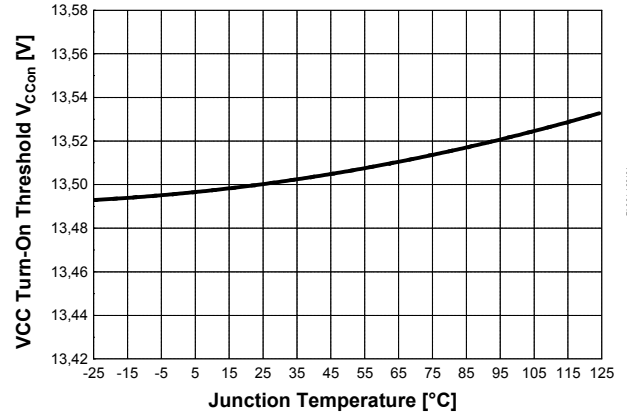
Figure 26 VCC Turn-On Threshold V_{VCCon} vs. T_j
