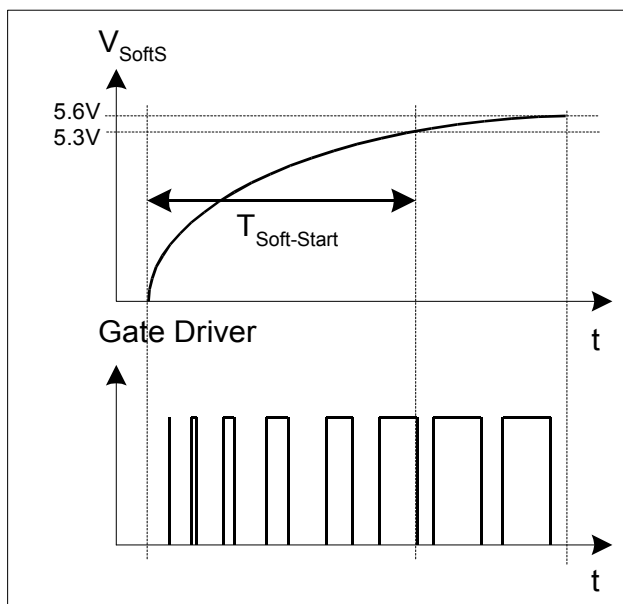
Figure 9 Soft-Start Phase
