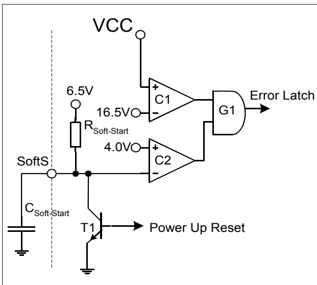
Figure 22 Overvoltage Detection
