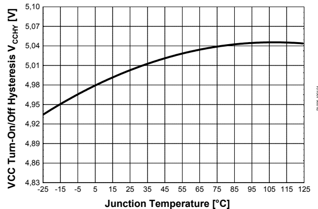
Figure 28 VCC Turn-On/Off Hysteresis V_{VCCHY} vs. T_j
