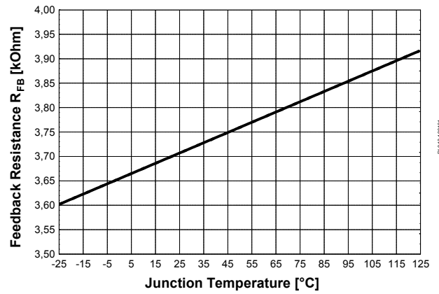
Figure 38 Feedback Resistance R_{FB} vs. T_j
