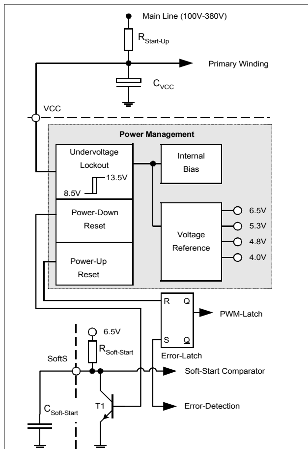
Figure 3 Power Management
