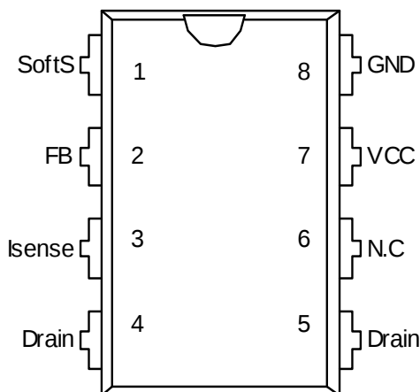
Figure 1 Pin Configuration PG-DIP-8 (top view)
