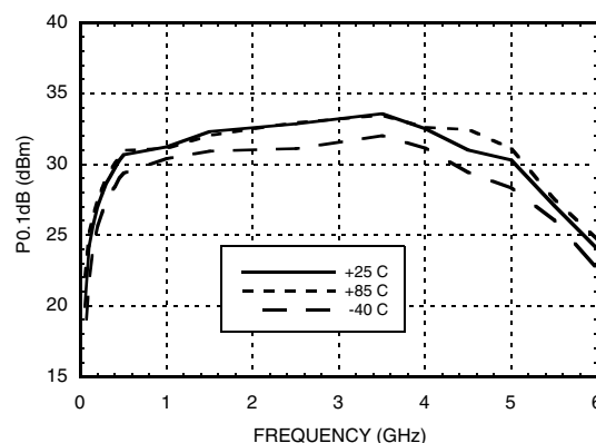
P0.1dB vs. Temperature, Min. Attn State [2]
