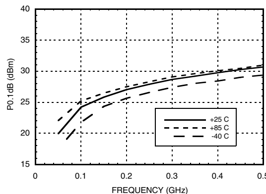
P0.1dB vs. Temperature, Min. Attn State [2] (Low Frequency Detail)
