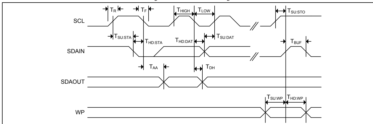
Figure 5-11. Bus Timing
