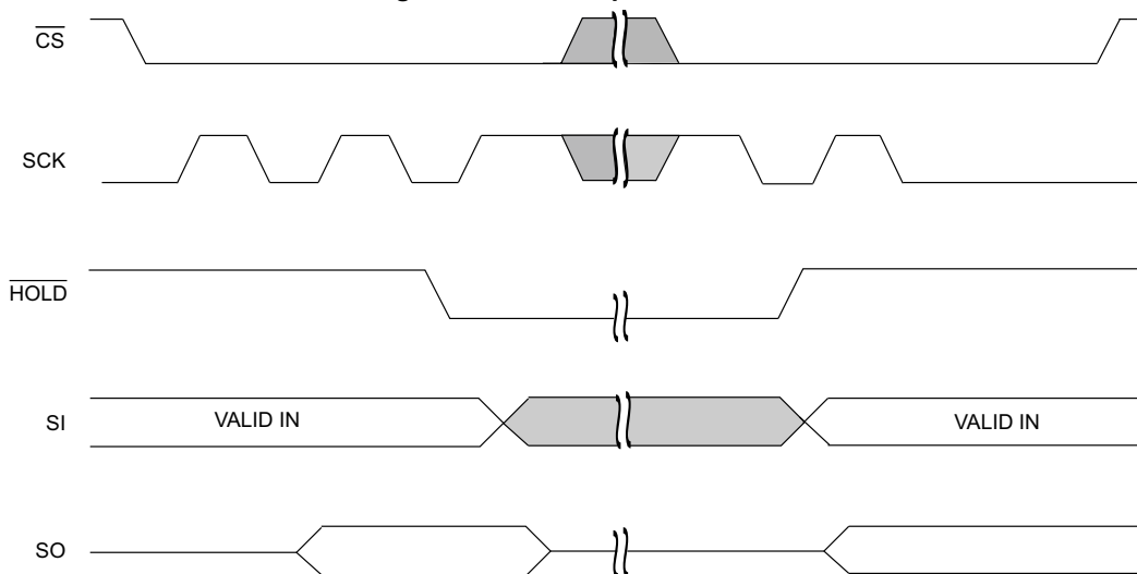
Figure 12. \overline{\text{HOLD}} Operation [2]
