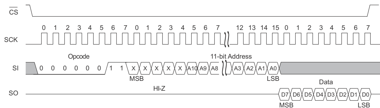
Figure 11. Memory Read
