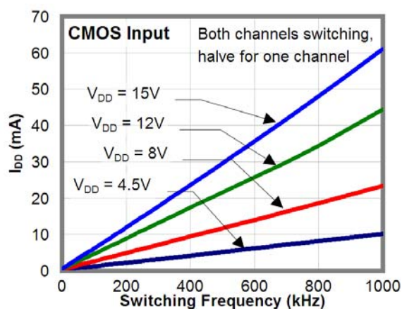
Figure 18. I_{DD} (1 nF Load) vs. Frequency
