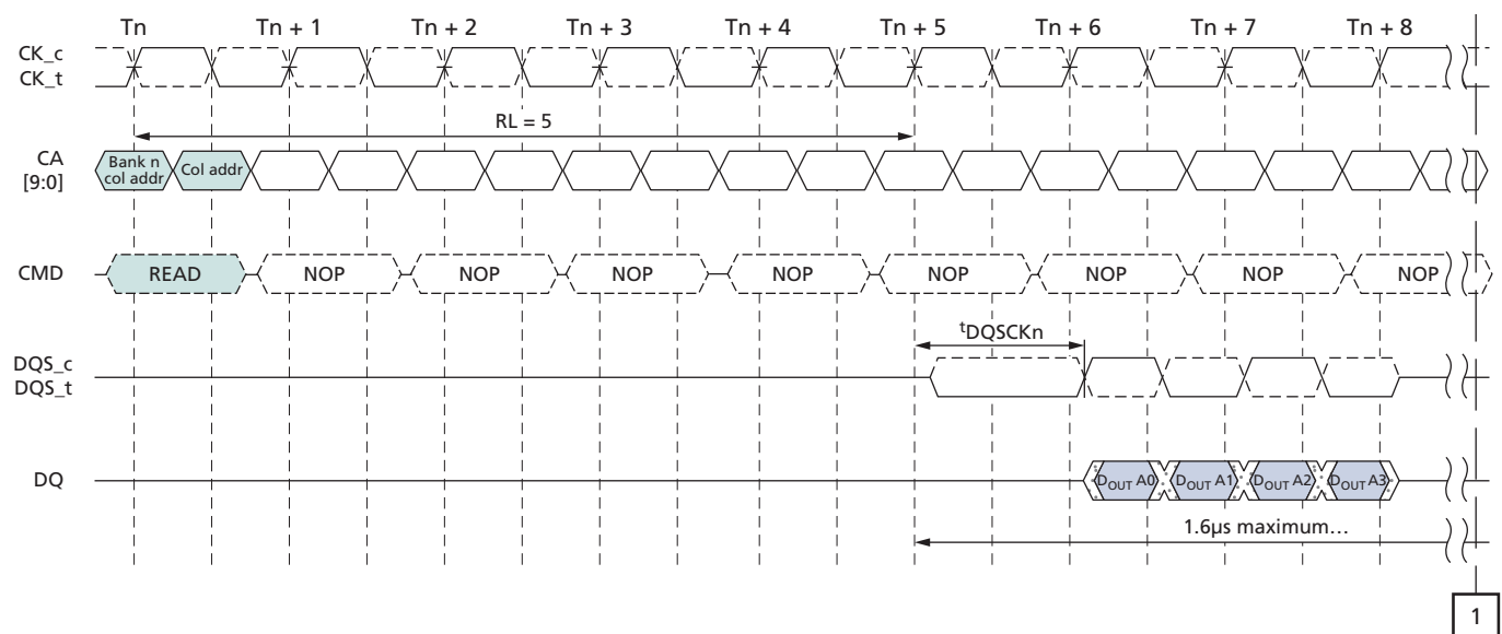
Figure 27: t_{DQSKDM} Timing
