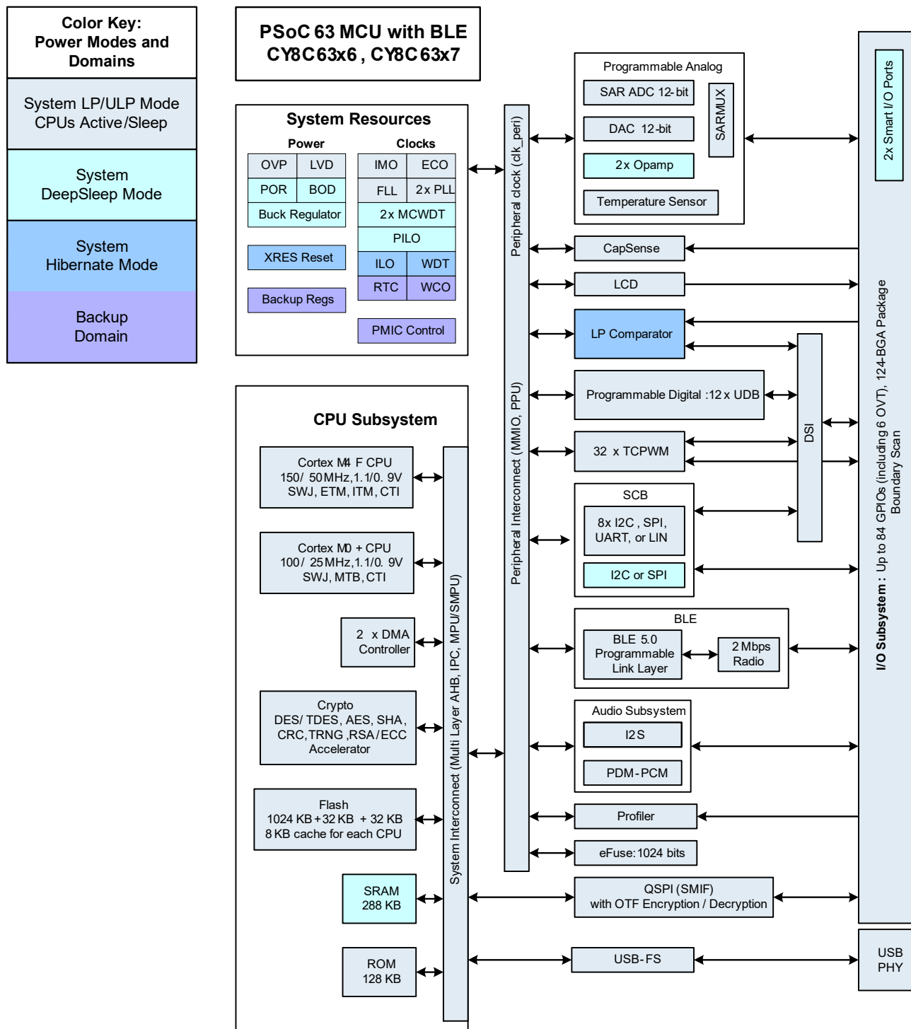
Figure 3. Block Diagram
