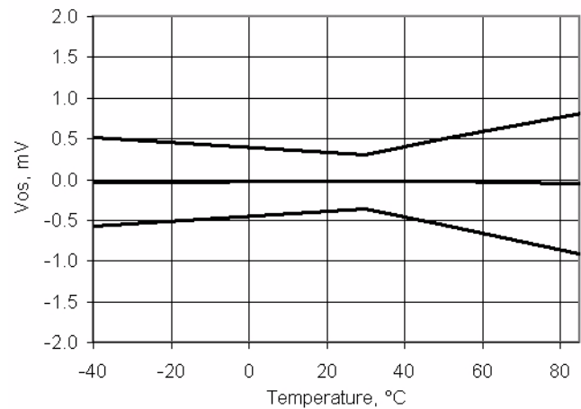
Figure 11-25. Opamp Voffset vs Temperature, V_{DDA} = 5\text{ V}
