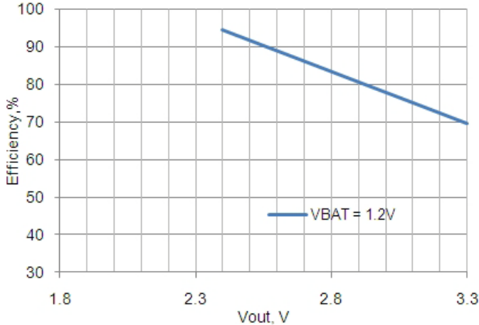
Figure 11-10. Efficiency vs V_{\text{OUT}} I_{\text{OUT}} = 75 \text{ mA} , V_{\text{BAT}} = 1.2 \text{ V}
