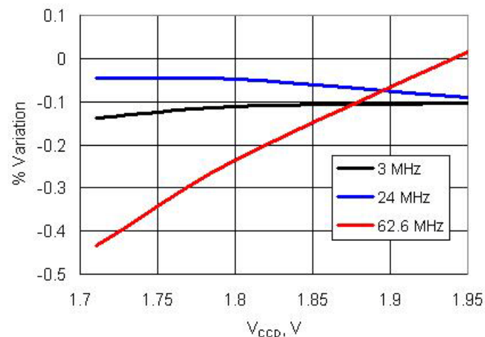
Figure 11-71. IMO Frequency Variation vs. V CC
