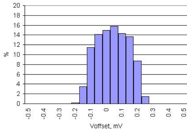
Figure 11-24. Opamp Voffset Histogram, 3388 samples/847 parts, 25\text{ }^{\circ}\text{C} , V_{DDA} = 5\text{ V}
