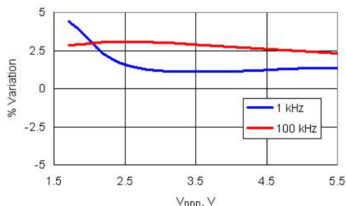
Figure 11-73. ILO Frequency Variation vs. V_{DD}
