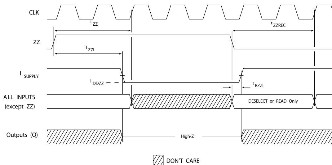
Figure 7. ZZ Mode Timing [31, 32]
