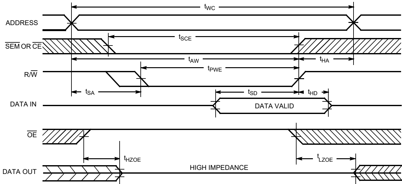
Figure 8. Write Cycle No. 2 ( \text{R}/\overline{\text{W}} Three-state Data I/Os (Either Port)) [20, 22, 23]
