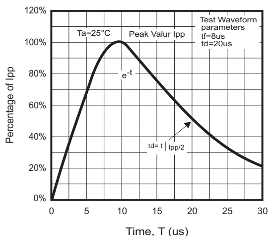
Fig.1 - 8/20 \mu\text{s} Peak Pulse Current
