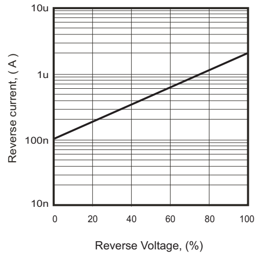
Fig.2 - Reverse Characteristics
