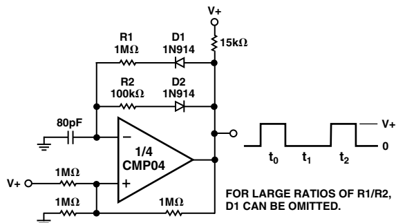
Figure 12. Pulse Generator
