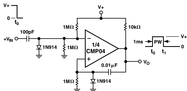
Figure 10. One-Shot Multivibrator
