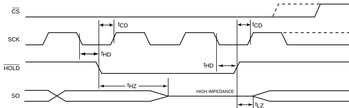
Figure 10. \overline{\text{HOLD}} Timing
