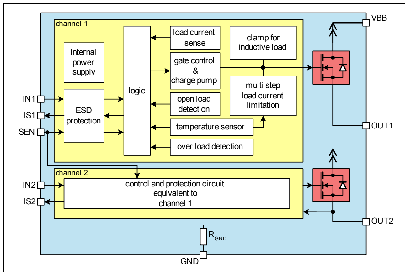
Figure 1 Block Diagram
