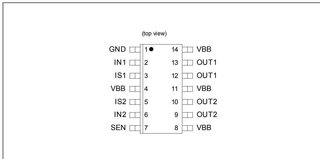
Figure 3 Pin Configuration PG-DSO-14-32
