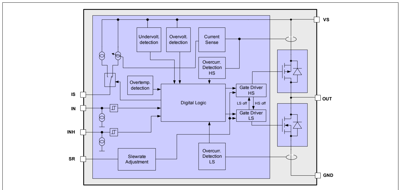
Figure 1 Block Diagram
