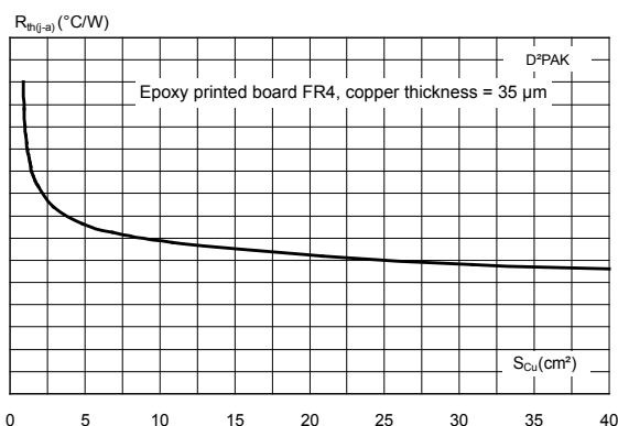
Figure 11. D 2 PAK thermal resistance junction to ambient versus copper surface under tab
