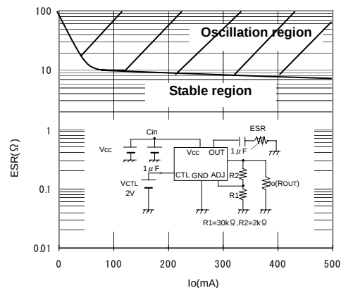
Fig.25 ESR-Io Characteristics
