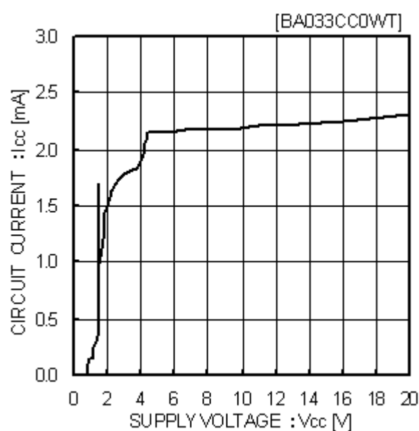
Fig.3 Circuit current
