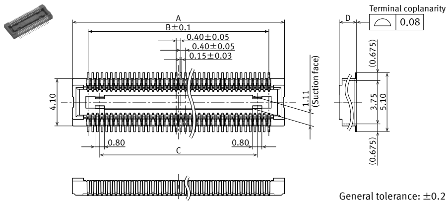
External dimensions
