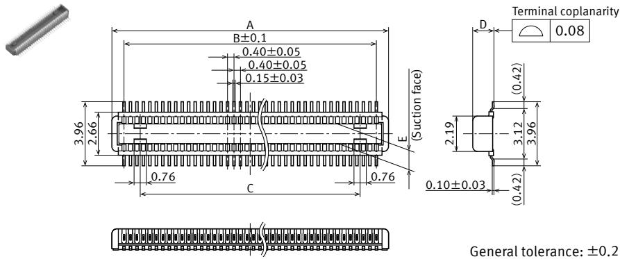
External dimensions
