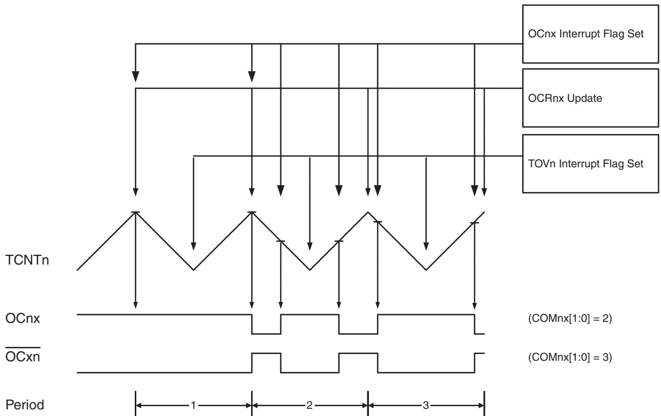
Figure 11-7. Phase Correct PWM Mode, Timing Diagram
