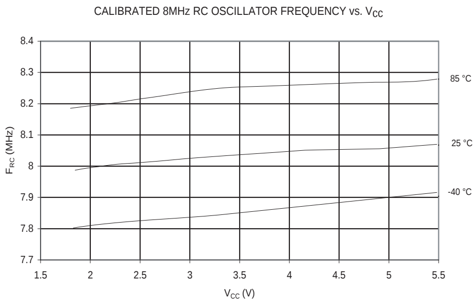
Figure 132. Calibrated 8 MHz RC Oscillator Frequency vs. V_{CC}
