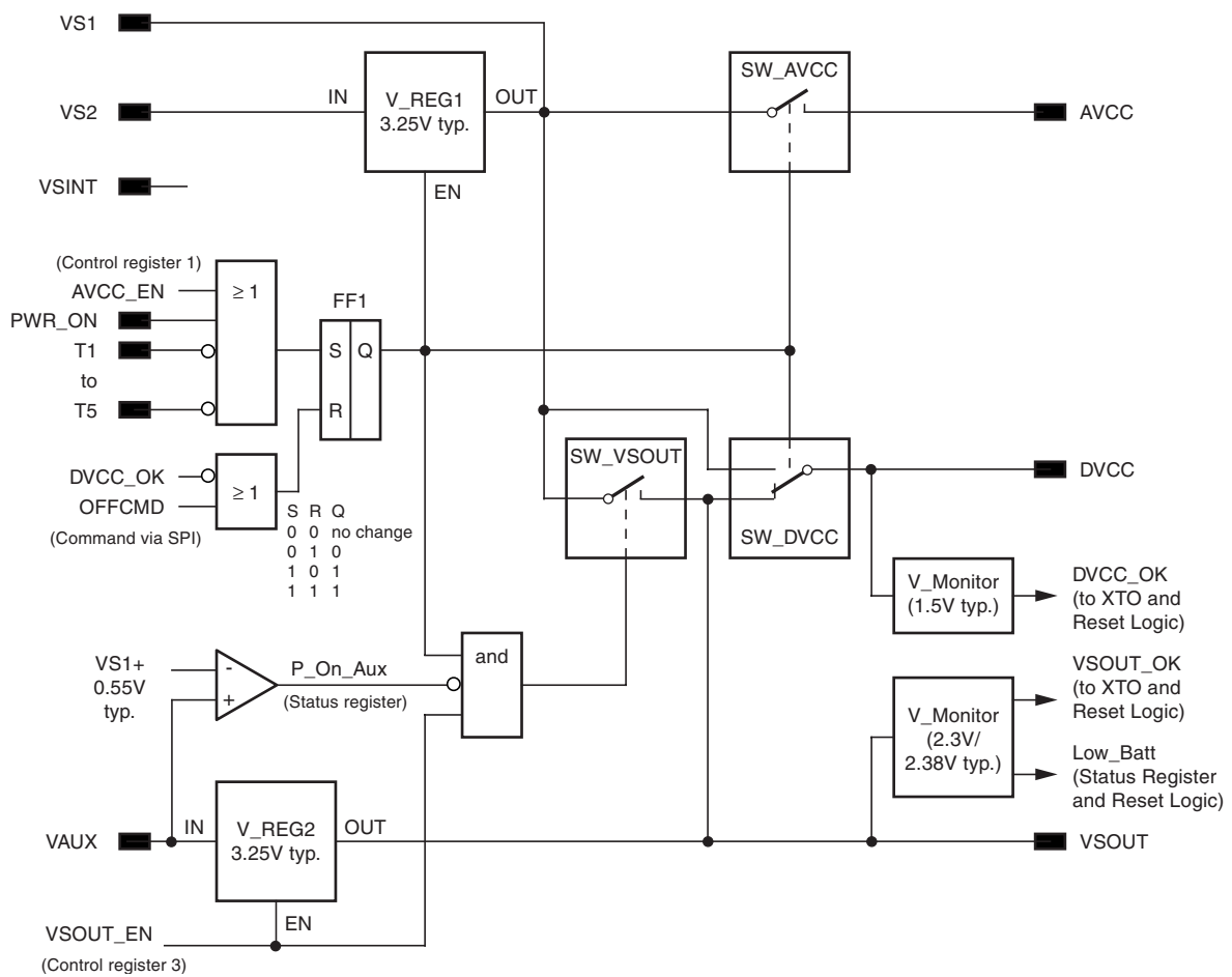
Figure 7-1. Power Supply
