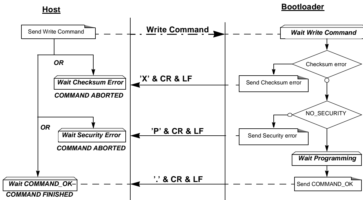
Figure 42. Write/Program Flow
