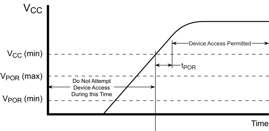
Figure 8-2. Power-Up Timing
