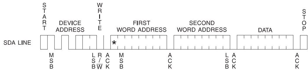
Figure 7. Byte Write
