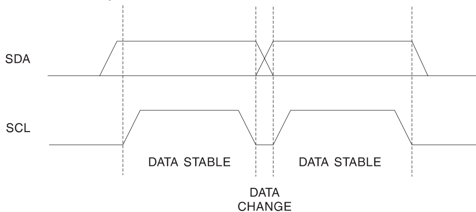
Figure 3. Data Validity
