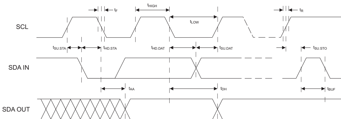
Figure 8-1. Bus Timing
