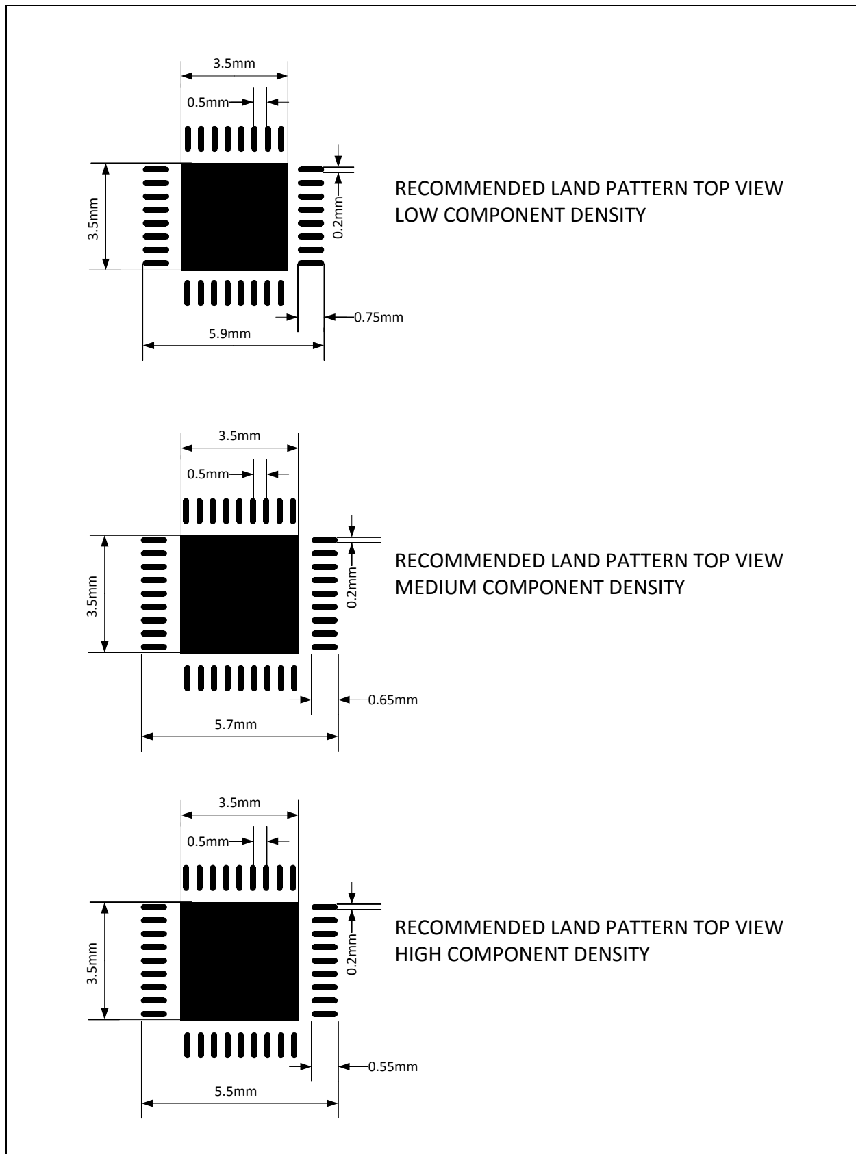
Figure 112: AS3415 PCB Pad Layout Recommendation
