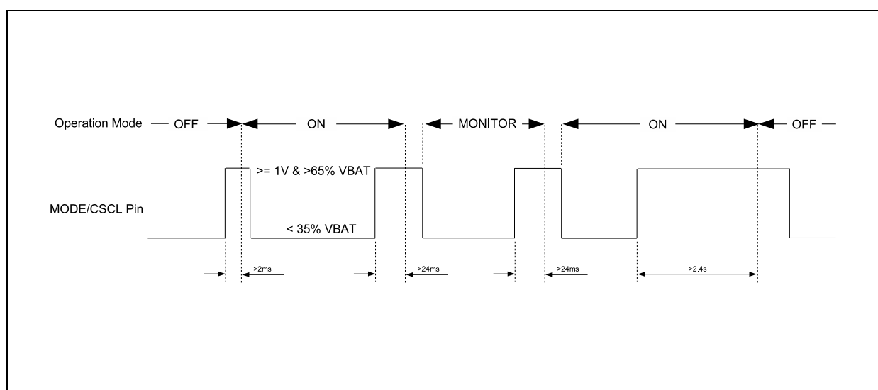
Figure 59: Push Button Mode Timing Diagram
