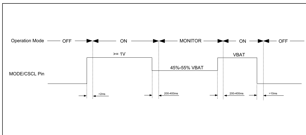
Figure 55: Full Slider Mode Timing Diagram
