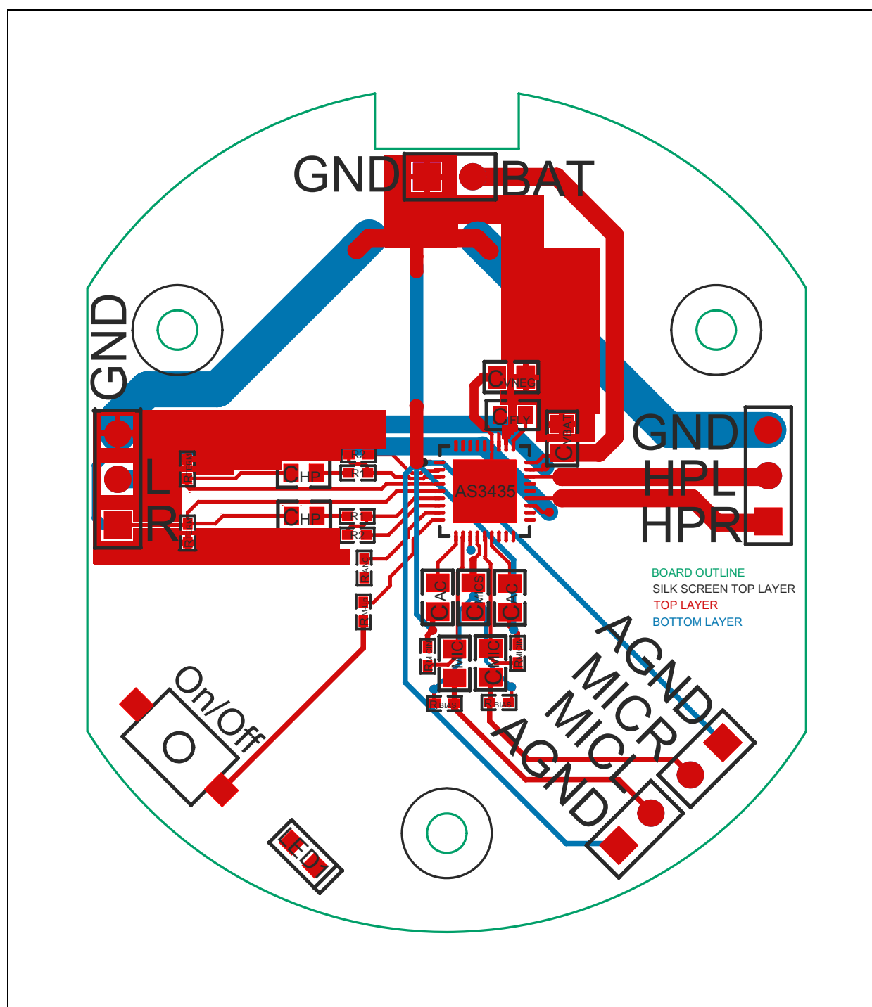
Figure 110: AS3435 Over the Ear Layout Example
