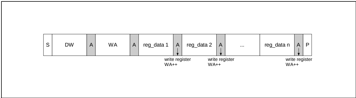
Figure 78: Page Write
