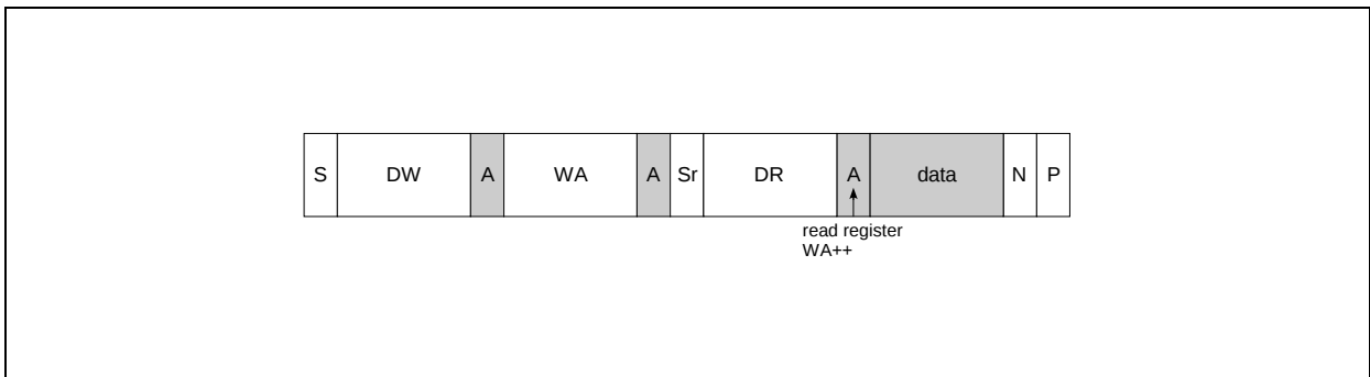
Figure 79: Random Read
