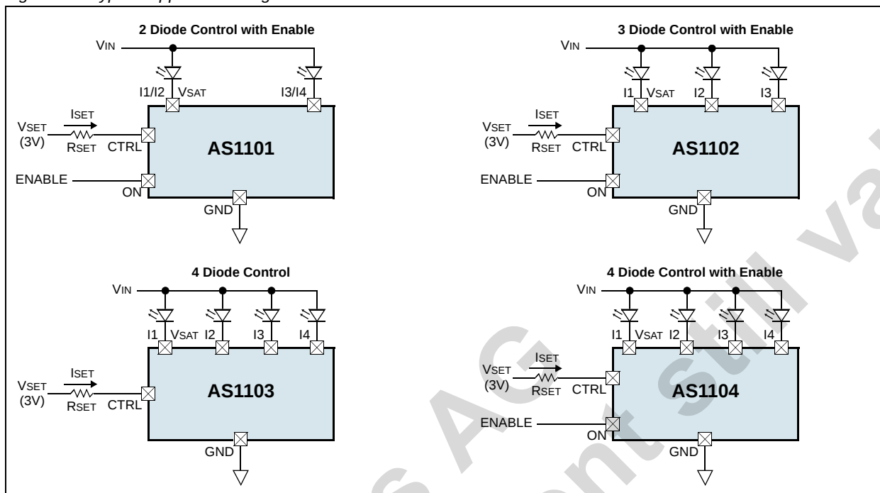
Figure 19. Typical Application Diagrams
