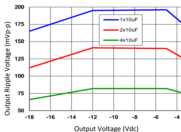
Figure 66. Output ripple with 1x10µF, 2x10µF or 4x10µF output ceramic capacitors (max load).
