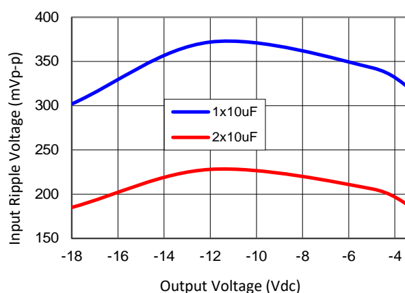
Figure 65. Input ripple voltage with 1x10 µF or 2x10 µF input ceramic capacitors (max load).
