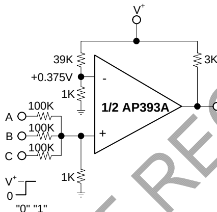
AND Gate
