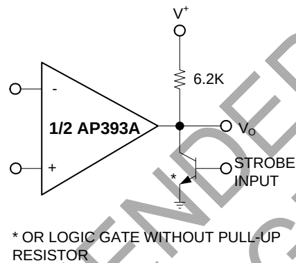
Output Strobing
