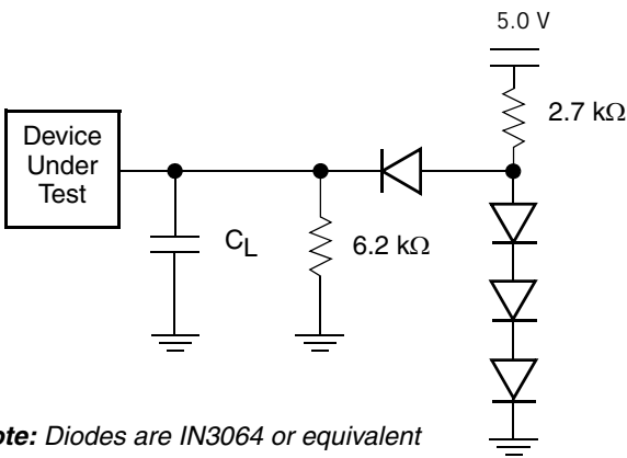
Figure 8. Test Setup
