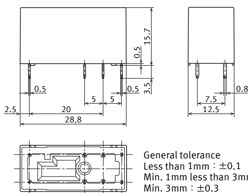
External dimensions
