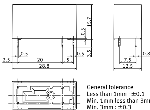
External dimensions
