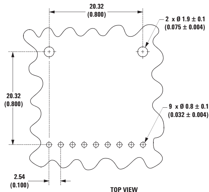
Figure 8. Recommended Board Layout Hole Pattern
