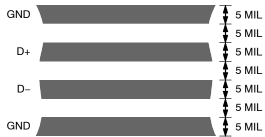
Figure 22. Typical Arrangement of Signal Tracks
