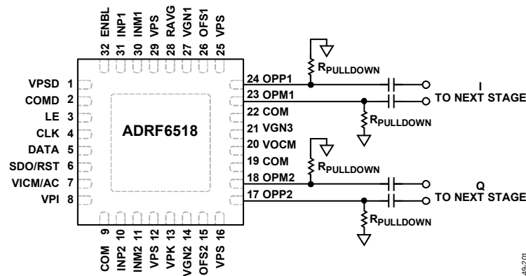
Figure 85. Pull-Down Resistors
